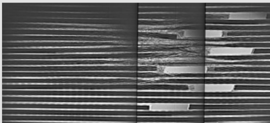
X-ray of 12 damaged/corroded cables approximately 1 foot from left edge in middle of splice.
